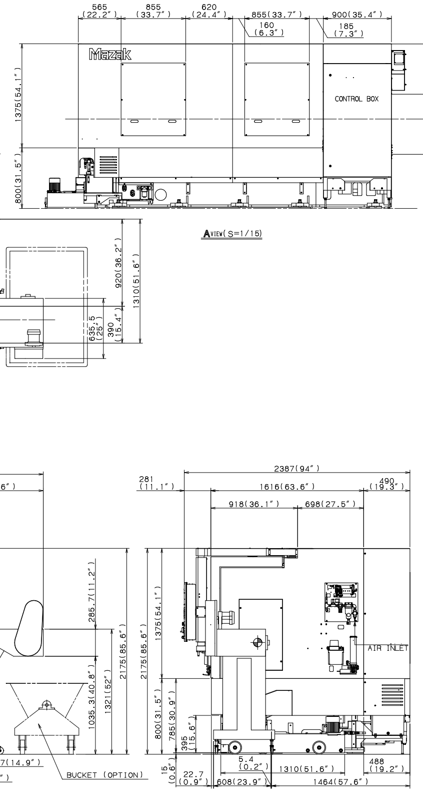
EXTERNAL DIMENSIONS – QUICK TURN 350, 350M, 350MY – 1500U (FOR REFERENCE ONLY)
